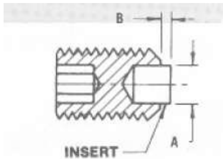
SET SCREW WITH NYLON/BRASS TIPPED.
